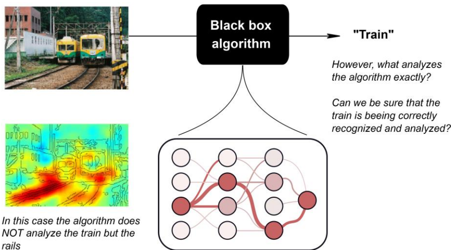
The method developed by Fraunhofer HHI and TU Berlin visualizes the analysis of the black box algorithm
